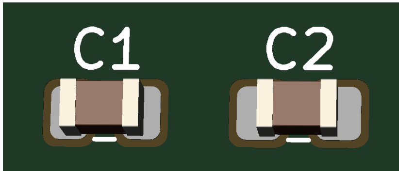
Figure 14 - Minimum Ratio (C1 - Left) & Larger Ratio (C2 - Right) – Both Acceptable
