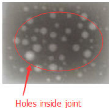
Figure 27 – X-Ray Image of Solder Joint Voids
